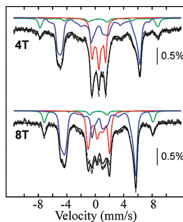
FIGURE 5: Mössbauer spectra (at 4.2 K) of the product of the reaction of free \text{Mn}^{\text{IV}}/\text{Fe}^{\text{III}}\text{-}\beta_2 and HU recorded in external magnetic fields of 4 T (top) and 8 T (bottom) applied parallel to the \gamma -beam. \beta subunit (3.0 mM monomer containing 0.75 equiv \text{Mn}^{\text{IV}}/\text{Fe}^{\text{III}} cluster per monomer) was incubated with 60 mM HU at ambient temperature for 25 min before being frozen. The contributions of \text{Mn}^{\text{IV}}/\text{Fe}^{\text{III}}\text{-}\beta_2 (57% intensity), the diamagnetic \text{Fe}^{\text{III}} -containing cluster (33% intensity), and the mononuclear high-spin \text{Fe}^{\text{III}} impurity (10% intensity) are shown as blue, red, and green lines, respectively. Simulation parameters are as follows: S = 5/2 , D = -0.38 \text{ cm}^{-1} , E/D = 0.31 , \mathbf{g} = (2.0, 2.0, 2.0) , \Delta E_Q = 0.56 \text{ mm/s} , \delta = 0.46 \text{ mm/s} , \mathbf{a}_{\text{Fe}}/\mathbf{g}_N\beta_N = (-22, -22, -22) \text{ T} , \eta = -0.19 (green lines); S = 0 , \Delta E_Q = -0.88 \text{ mm/s} , \delta = 0.49 \text{ mm/s} , \eta = -0.43 (red lines); S = 1 , D = -1.9 \text{ cm}^{-1} , E/D = 0.33 , \mathbf{g} = (2.0, 2.0, 2.0) , \Delta E_Q = -1.38 \text{ mm/s} , \delta = 0.52 \text{ mm/s} , \mathbf{a}_{\text{Fe}}/\mathbf{g}_N\beta_N = (-39.0, -39.2, -37.6) \text{ T} , \eta = -0.23 (blue lines). The black lines overlaid with the experimental spectra are the summations of the three components.
