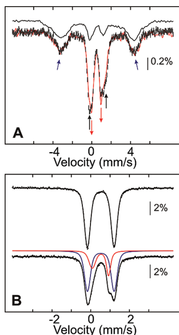
FIGURE 4: Mössbauer spectra illustrating the different outcomes of the reaction of \text{Mn}^{\text{IV}}/\text{Fe}^{\text{III}}\text{-}\beta_2 with HU. (A) Mössbauer spectra (at 4.2 K and 53 mT) of samples in which \text{Mn}^{\text{IV}}/\text{Fe}^{\text{III}}\text{-}\beta_2 (800 \mu\text{M} \beta and 0.75 equiv of \text{Mn}^{\text{IV}}/\text{Fe}^{\text{III}} cluster) was reacted with 20 mM HU at ambient temperature for 1 min (black hashed vertical bars) or 10 min (red solid line) in the presence of 1.2 mM \alpha , 10 mM DTT, 1 mM ATP, and 10 mM CDP. The black solid line is the spectrum of the heterogeneous \text{Mn}^{\text{IV}}/\text{Fe}^{\text{III}}\text{-}\beta_2 state (49). The black and red arrows indicate the conversion of the \text{Mn}^{\text{IV}}/\text{Fe}^{\text{III}} form to the new \text{Fe}^{\text{III}} -containing complex. The blue arrows indicate the outer lines of the magnetically split subspectrum of the \text{Mn}^{\text{III}}/\text{Fe}^{\text{III}} cluster ( \sim 45\% of the total intensity). The amounts of \text{Mn}^{\text{III}}/\text{Fe}^{\text{III}} cluster in the two samples are identical within experimental uncertainty. (B) Mössbauer spectra (at 4.2 K and zero field) of samples prepared by treatment of \text{Mn}^{\text{IV}}/\text{Fe}^{\text{III}}\text{-}\beta_2 (top) with 20 mM HU for 30 min at ambient temperature (bottom). The solid lines on top are simulations as indicated in the text. The blue and red lines represent the contributions of the \text{Mn}^{\text{IV}}/\text{Fe}^{\text{III}} cluster and the new \text{Fe}^{\text{III}} -containing, diamagnetic species, respectively.
