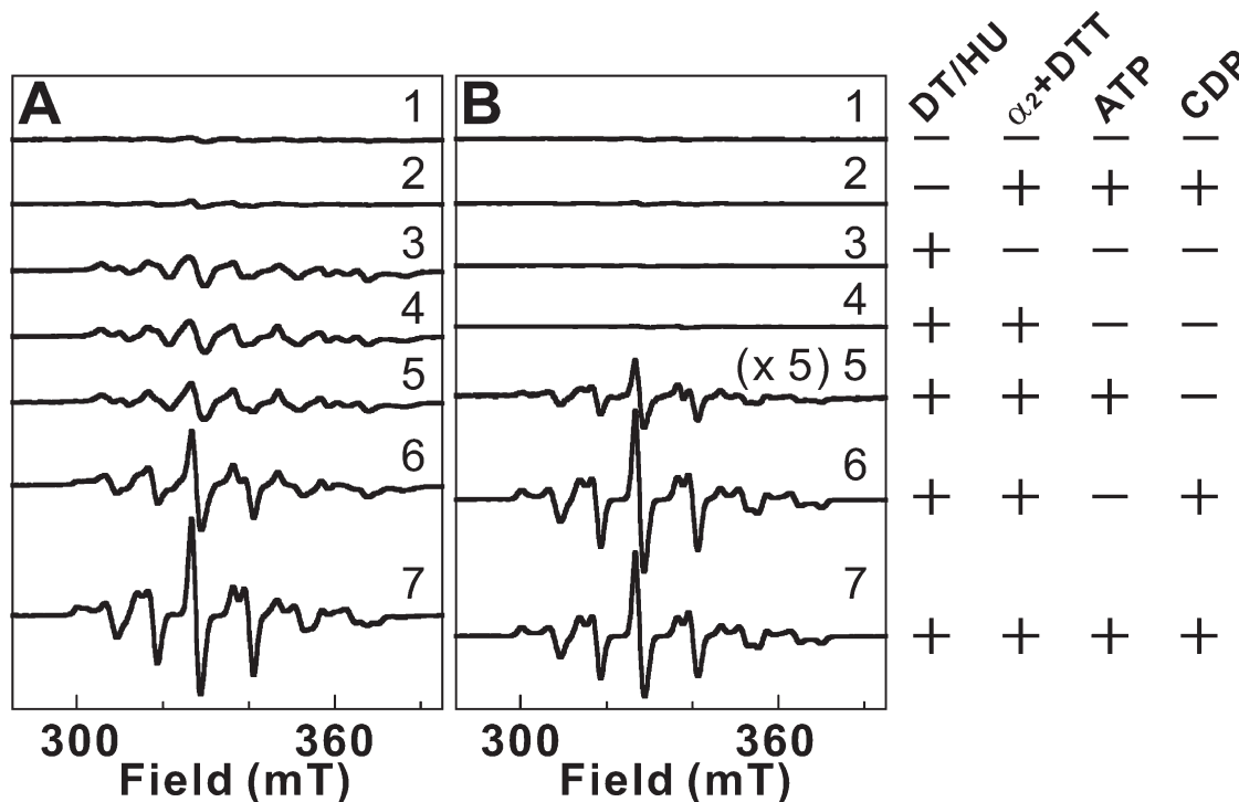
FIGURE 2: X-Band EPR spectra showing the requirements for formation of the homogeneous \text{Mn}^{\text{IV}}/\text{Fe}^{\text{III}} state in \beta_2 upon treatment of \text{Mn}^{\text{IV}}/\text{Fe}^{\text{III}}\text{-}\beta_2 with either DT (A) or HU (B). 300\text{ }\mu\text{M} \beta monomer containing 0.75 equiv of \text{Mn}^{\text{IV}}/\text{Fe}^{\text{III}} cluster was present in all samples. The presence (+) or absence (—) of the various other components is indicated on the right side of the corresponding spectrum. When included, the other components were present at concentrations of 900\text{ }\mu\text{M} \alpha_2 , 10 mM DTT, 4 mM CDP, 1 mM ATP, 20 mM DT, and 20 mM HU. All components except DT or HU were mixed, and the reductant was quickly added. Samples were incubated for 5 min at ambient temperature in the absence of \text{O}_2 before being frozen. Spectra were acquired with a temperature of 14.0 \pm 0.2\text{ K} , a microwave frequency of 9.45 GHz, a microwave power of 200\text{ }\mu\text{W} , a modulation frequency of 100 kHz, a modulation amplitude of 1 mT, a scan time of 167 s, and a time constant of 167 ms.
