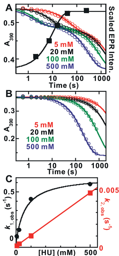
FIGURE 3: (A) Kinetics of the absorbance changes at 390 nm (left y-axis) during the reaction of Mn IV /Fe III -β 2 with HU in the presence of α 2 , CDP, and ATP at ambient temperature (22 ± 2 °C) and relative intensities of the EPR signal characteristic of the homogeneous Mn III /Fe III -β 2 state (right y-axis). A solution containing 400 μM β monomer (0.75 equiv Mn IV /Fe III cluster), 800 μM α monomer, 20 mM DTT and 2 mM ATP was mixed with an equal volume of reaction buffer containing 8 mM CDP and HU at a concentration appropriate to give the HU concentration listed in the figure (after mixing). The solid lines overlaid are fits of eq 1 to the data. The black squares are the EPR signal intensities extracted from the spectra shown in Figure S1 of the Supporting Information. The solid line is a fit of a single-exponential phase to the data, which gives a rate constant of 0.10 ± 0.03 s -1 . (B) Kinetics of the reaction of Mn IV /Fe III -β 2 with HU. The reaction was initiated in the same fashion described above but in the absence of α 2 , CDP, ATP, and DTT. (C) Dependence of the apparent first-order rate constants for the reactions on the concentration of HU. k 1,obs (black circles) was extracted from the fast phase in panel A, and the overlaid solid line is the hyperbolic fit to the data, which gives a limiting reduction rate constant (asymptote of the hyperbolic fit) of 0.7 ± 0.1 s -1 . k 2,obs (red squares) was extracted from the reactions in panel B. The linear fit gives the second-order rate constant (slope) of (9.0 ± 2.0) × 10 -3 M -1 s -1 .
