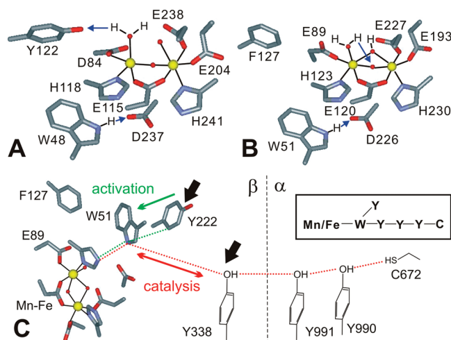
FIGURE 1: Structural representations of the \text{Fe}_2^{\text{III/III}} forms of Ec \beta_2 (A) and Ct \beta_2 (B) generated from the crystallographic coordinates available in Protein Data Bank entries 1MXR and 1SYY, respectively. Proposed proton transfer steps associated with gating of PCET are indicated with blue arrows in panels A and B. In panel C, the proposed electron transfer pathways of Ct RNR specific to catalysis (red dotted line) and activation of \beta_2 by formation of its \text{Mn}^{\text{IV}}/\text{Fe}^{\text{III}} cofactor (green dotted line) are shown. The black arrows indicate amino acid residues important in reduction of the \text{Mn}^{\text{IV}}/\text{Fe}^{\text{III}} - \beta_2 \cdot \alpha_2 \cdot \text{CDP} \cdot \text{ATP} complex to the \text{Mn}^{\text{III}}/\text{Fe}^{\text{III}} form by hydroxyurea. A symbolic scheme of the residues involved in electron transfer is shown in the inset.
