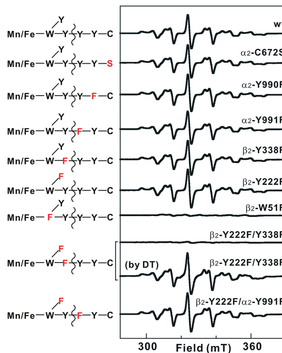
FIGURE 7: X-Band EPR spectra of samples prepared by reaction of wild-type or variant \text{Mn}^{\text{IV}}/\text{Fe}^{\text{III}}\text{-}\beta_2 with HU or DT in the presence of \alpha_2 (wild type or variant), CDP, and ATP. The corresponding schematic of the branched electron transfer pathways is shown at the left, with redox-active residues colored black and redox-inactive ones colored red. An \text{O}_2 -free solution containing 300 \mu\text{M} \beta monomer (0.75 equiv of \text{Mn}^{\text{IV}}/\text{Fe}^{\text{III}} cluster), 900 \mu\text{M} \alpha monomer, 4 mM CDP, 1 mM ATP, and 10 mM DTT was constituted. HU or DT was then added to a final concentration of 20 mM, and the solution was incubated for 5 min at ambient temperature before being frozen. Spectra were acquired with a temperature of 14.0 \pm 0.2 K, a microwave frequency of 9.38 GHz, a microwave power of 200 \mu\text{W} , a modulation frequency of 100 kHz, a modulation amplitude of 1 mT, a scan time of 20.97 s, and a time constant of 5.12 ms.
